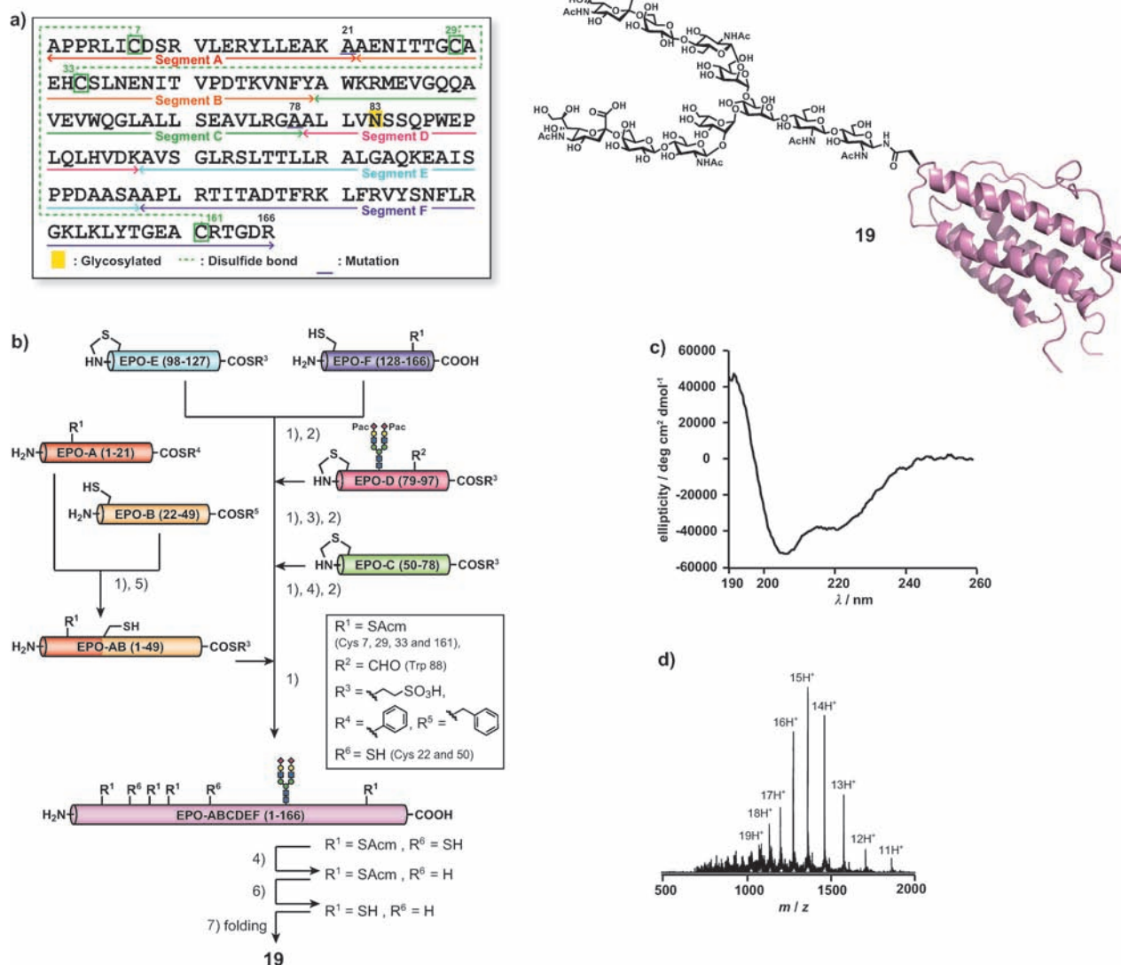
Figure 5. Synthesis of erythropoietin. a) Amino acid sequence and complete structure of the target EPO 19 . b) The synthesis of EPO with a human complex-type disialyloligosaccharide by chemical ligation and selective desulfurization: 1) ligation, 2) conversion of Thz into Cys with methoxyamine-HCl, 3) deprotection of formyl group of Trp and Pac group with piperidine, 4) desulfurization of cysteine, 5) thioester exchange with MESNa, 6) removal of AcM groups with AgOAc, 7) folding experiments under cysteine–cysteine redox conditions. c) CD spectrum of folded EPO 19 . d) Mass spectrum of folded EPO 19 .
