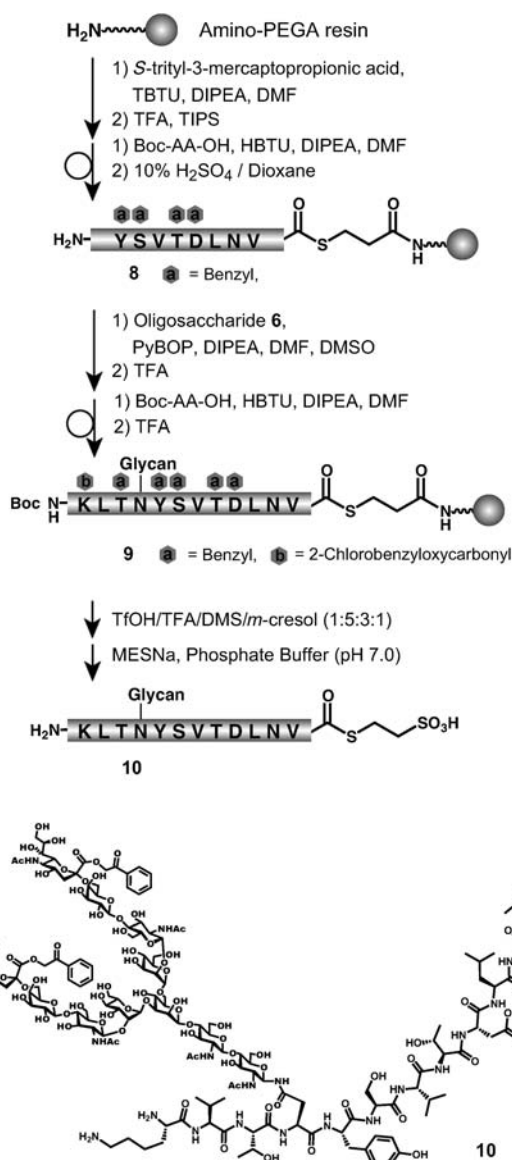
Scheme 2. Synthesis of sialylglycopeptide \alpha -thioester 10 . AA = amino acid. The arrows with the fused circle represent repeated coupling steps.
